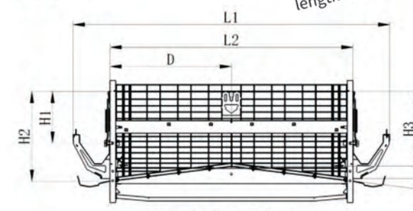
行车式H型商品蛋鸡笼 H type layer cage—traveling hopper
