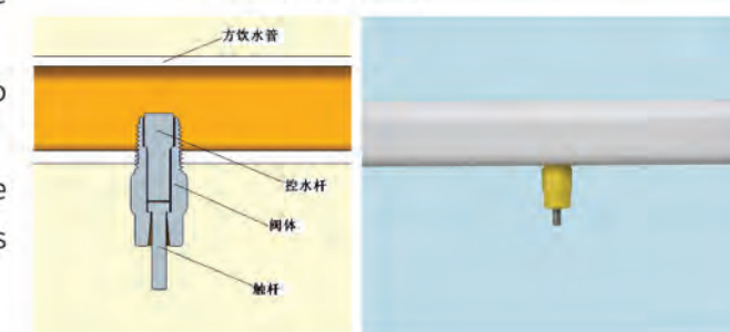
Cone valve drinker
