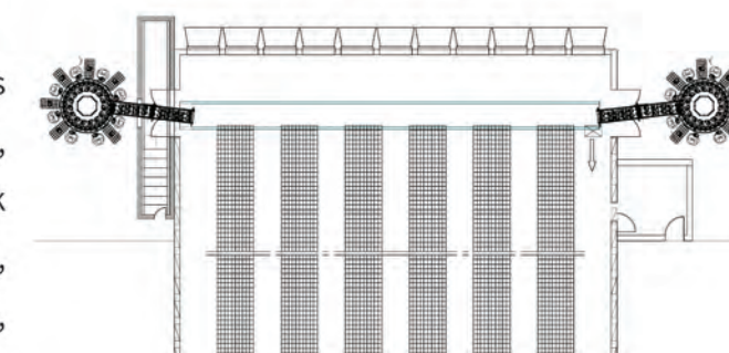
Two-way chick harvest diagram
