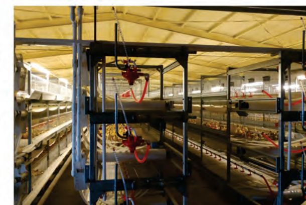
Cage front
