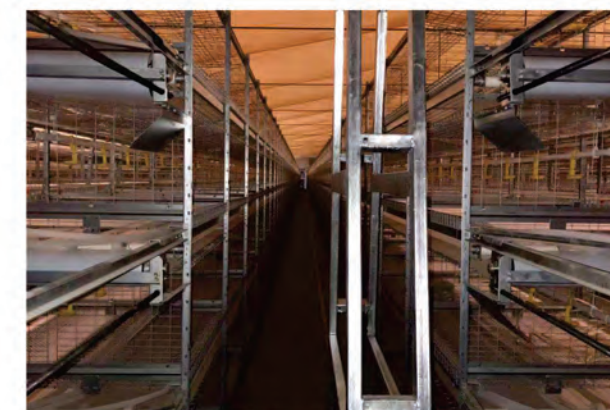
Seeder type traveling hopper feeder
