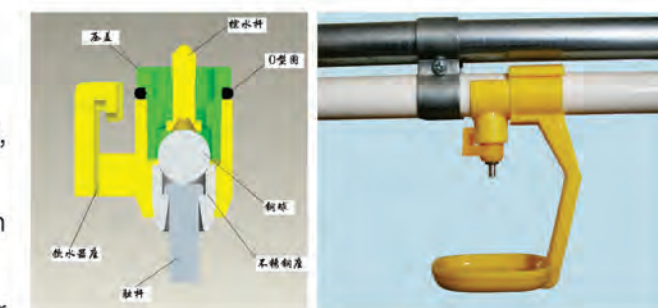
Ball valve drinker
